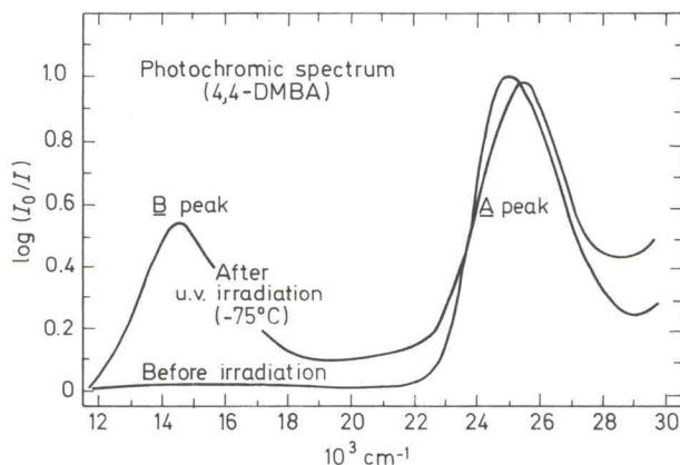
Figure 13. Spectra of unirradiated and irradiated 4,4'-DMBA in PMMA
